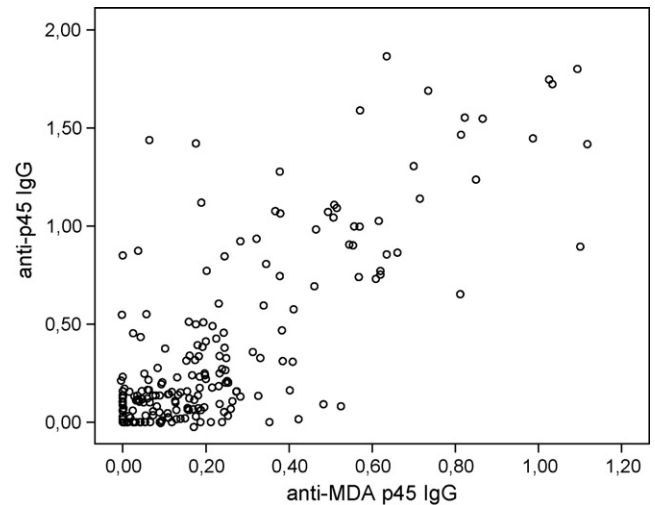
Fig. 1. Scatter plot demonstrating the association between plasma levels of autoantibodies against the native and MDA-modified p45 sequence of apo B-100.
